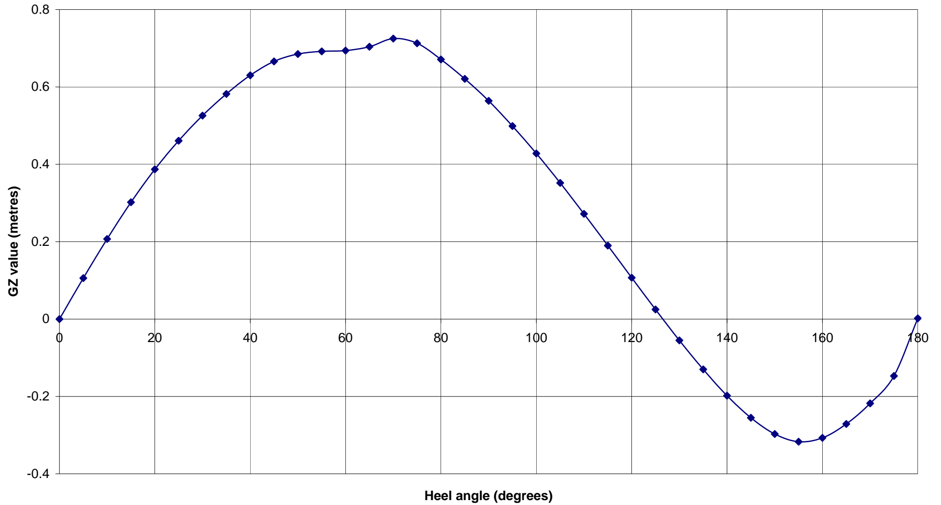
Impression 514 preliminary GZ curve
